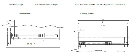
Installation dimensions
