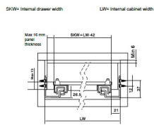
Installation dimensions
